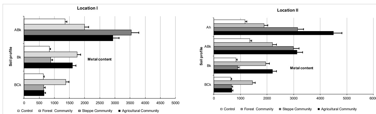
Figure 2. Iron content in soil profile under different plant communities
