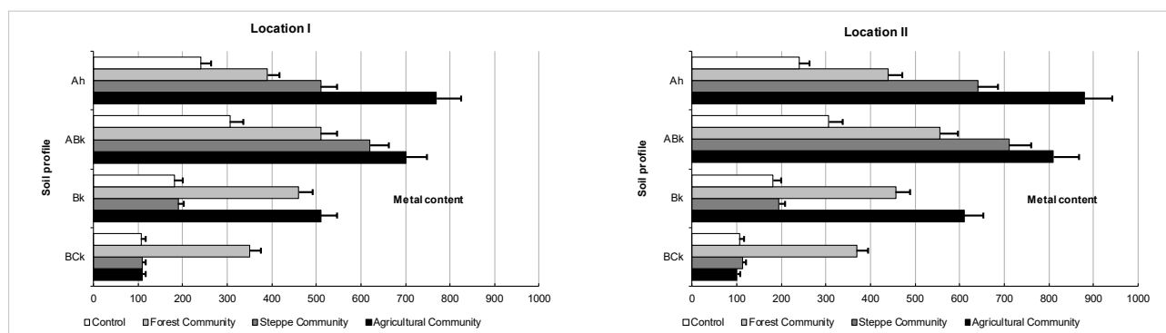
Figure 3. Manganese content in soil profile under different plant communities
