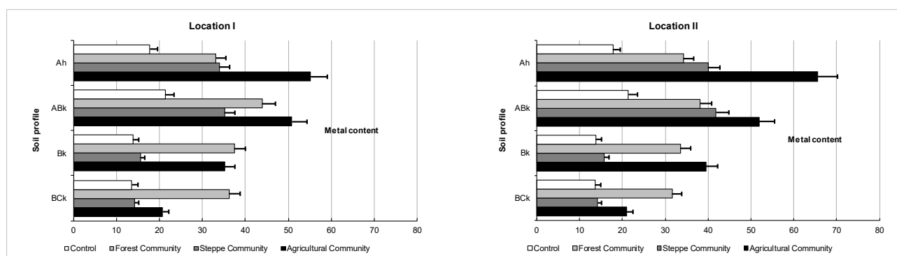
Figure 4. Zinc content in soil profile under different plant communities
